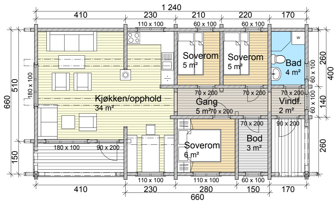
Grunnplan
